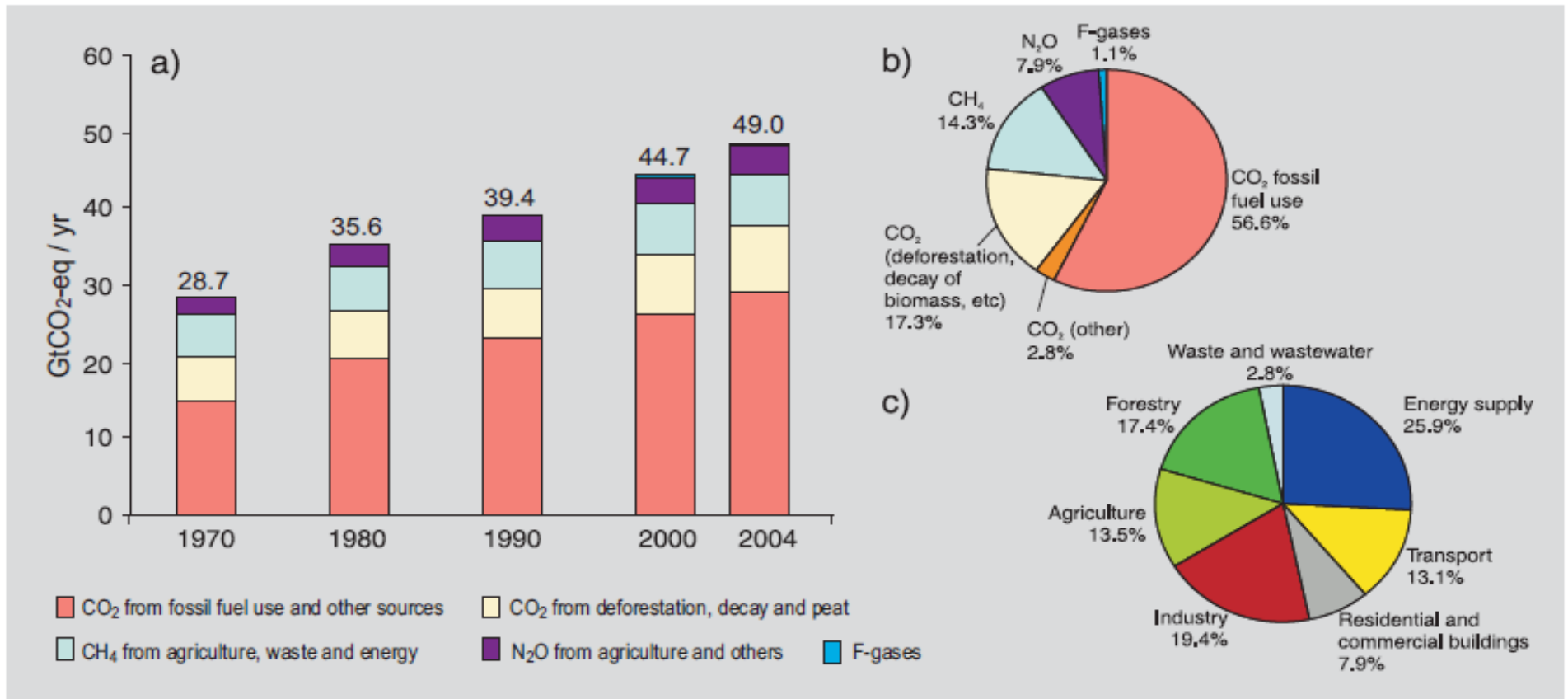
Figure SPM.3. (a) Global annual emissions of anthropogenic GHGs from 1970 to 2004. 5 (b) Share of different anthropogenic GHGs in total emissions in 2004 in terms of carbon dioxide equivalents (CO 2 -eq). (c) Share of different sectors in total anthropogenic GHG emissions in 2004 in terms of CO 2 -eq. (Forestry includes deforestation.) {Figure 2.1}
